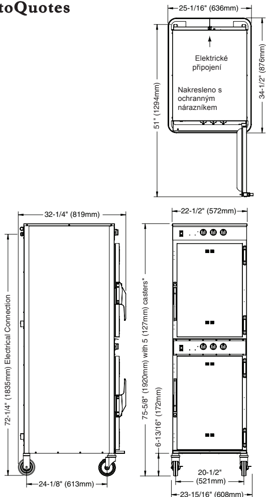
*74-1/4\" (1885mm) - with optional 3-1/2\" (89mm) casters *75-1/2\" (1917mm) - with optional 6\" (152mm) legs
